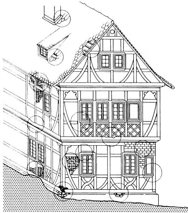
1 Main defect areas in half-timbered houses
